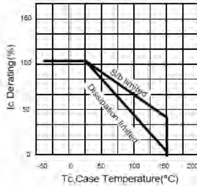
Fig.2 Derating curve of safe operating areas
