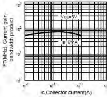
Fig.5 Current gain-bandwidth product
