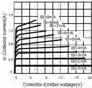
Fig.1 Static characteristics
