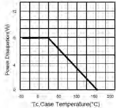
Fig.3 Power Derating
