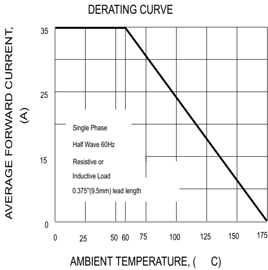
FIG.1-TYPICAL FORWARD CURRENT
