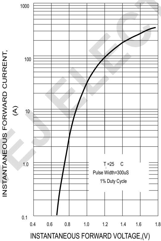
FIG.3-TYPICAL INSTANTANEOUS FORWARD CHARACTERISTICS
