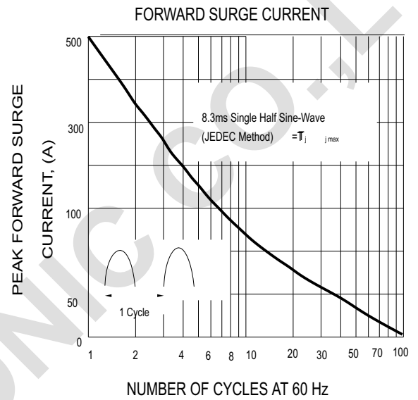
FIG.2-MAXIMUM NON-REPETITIVE PEAK
